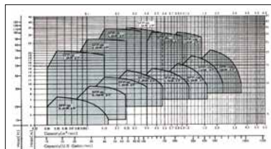
Model : SFP - (G)
